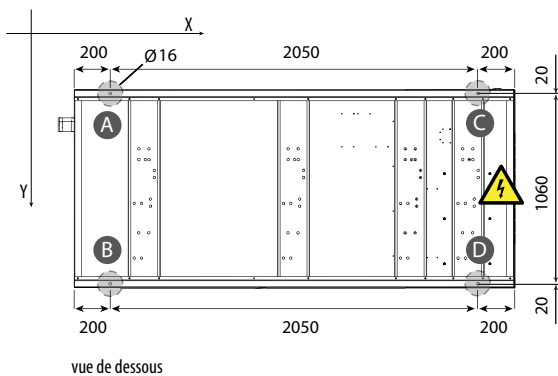
LAYOUT 1
