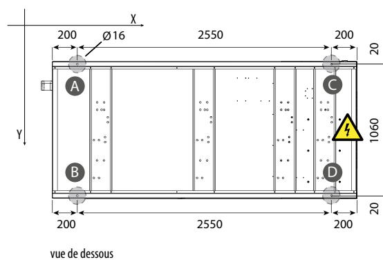
LAYOUT 2
